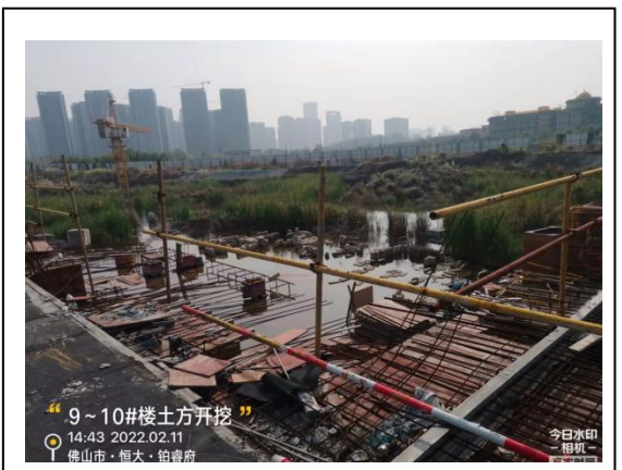
9~10#楼土方开挖
